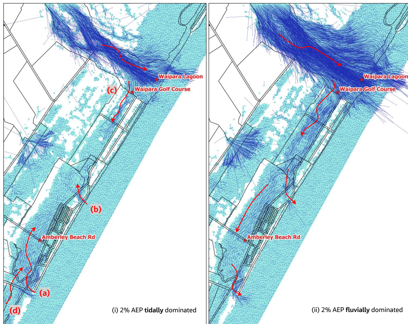
Figure 11: Model flood extents and velocities for (i) Scenario 7 (2% AEP tidally dominated event); and (ii) Scenario 8 (2% AEP fluvially dominated event), both with 0.5 m sea level rise, showing the main flood flow paths for Amberley Beach.
