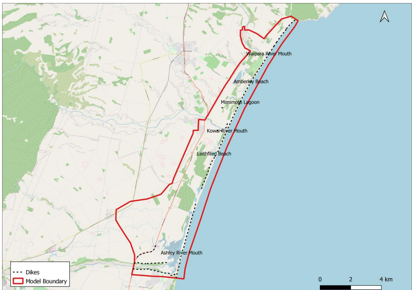
Figure 2 Model schematisation
