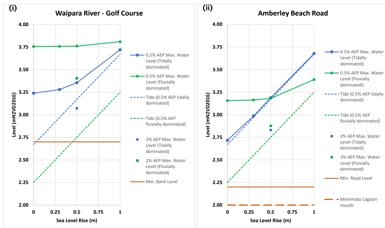
Figure 12: Model maximum water levels in (i) the Waipara River and (ii) at Amberley Beach Road for all scenarios simulated, showing the effect of sea level rise on tidally and fluvially dominated flood levels.
