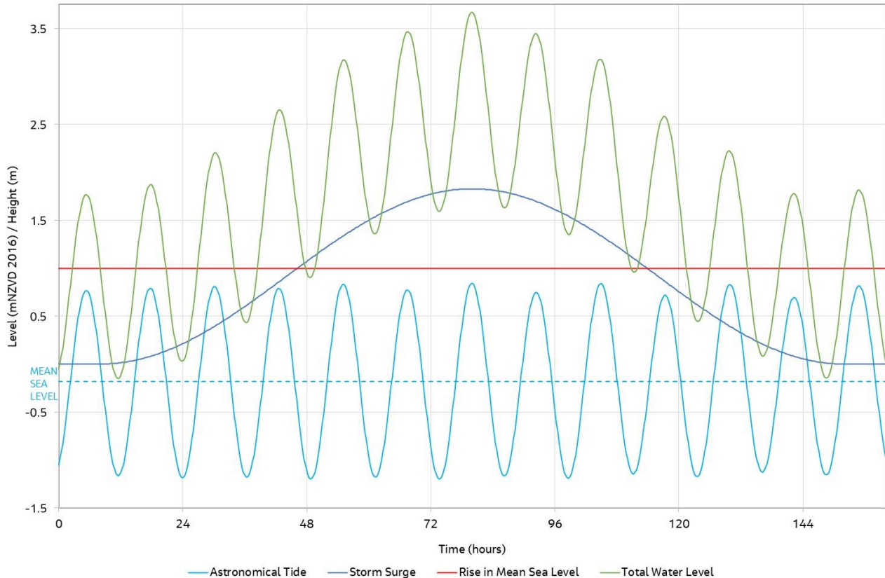
Figure 4: Development of model water level boundary for Scenario 7 (0.5% AEP sea level with 1m rise in mean sea level)
