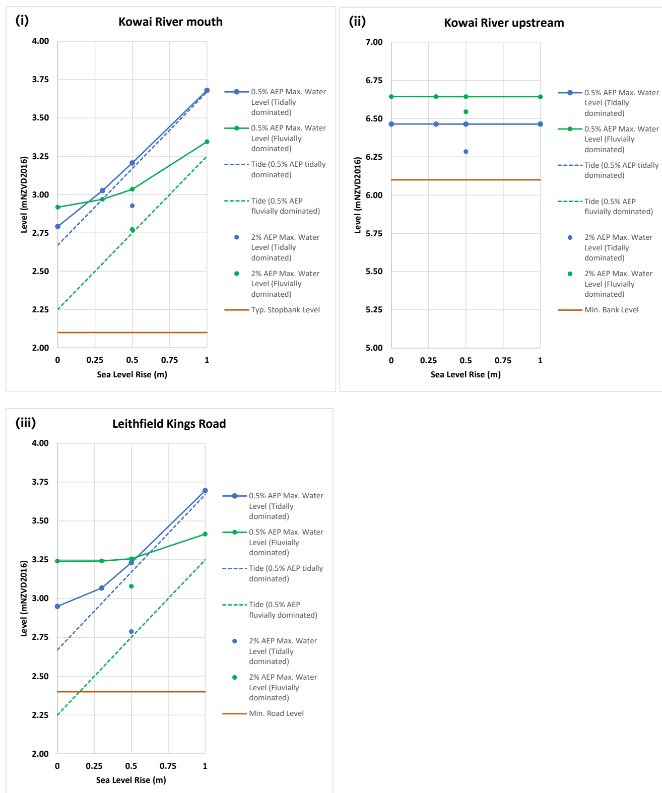
Figure 10: Model maximum water levels in (i) the mouth of the Kowai River; (ii) in the Kowai River further upstream; and (iii) at Kings Road for all scenarios simulated, showing the effect of sea level rise on tidally and fluviually dominated flood levels.
