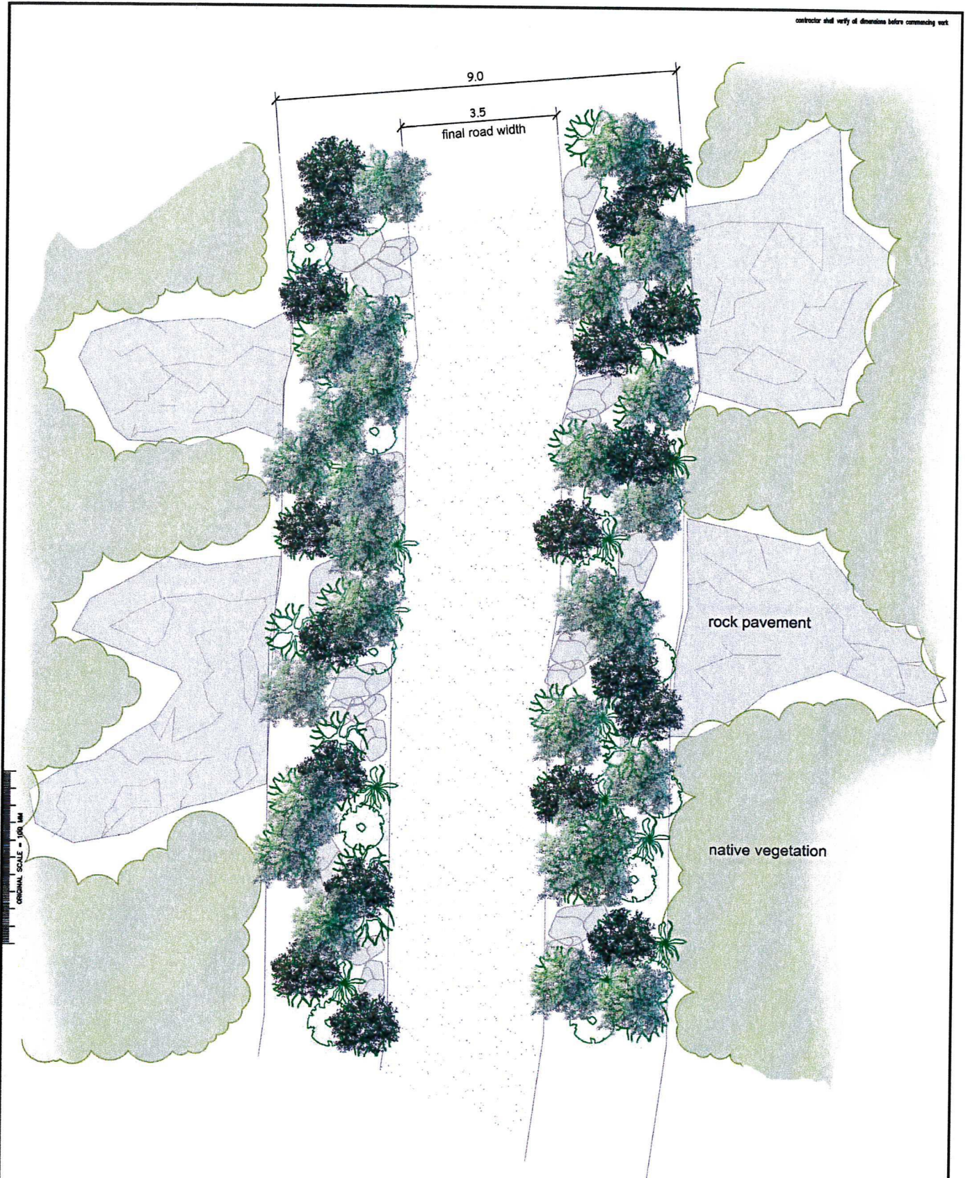
3. Plan view of completed road formation
